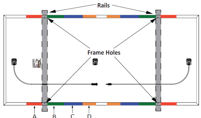
Figure 4: Mounting Zone Locations for Performance modules
